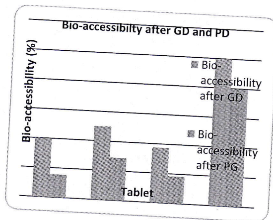
Fig 4 Bio-accessibility after Gastric digestion (GD) and Pancreatic digestion (PD)
