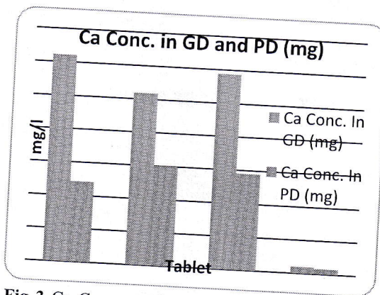
Fig 3 Ca Concentration in Gastric digestion (GD) and Pancreatic Digestion (PD).
